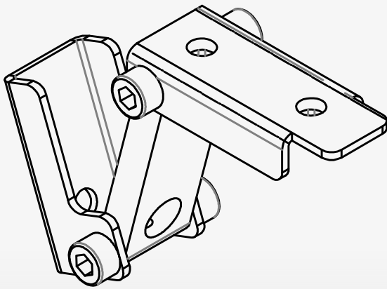
W2C-1 Clamp Assembly
