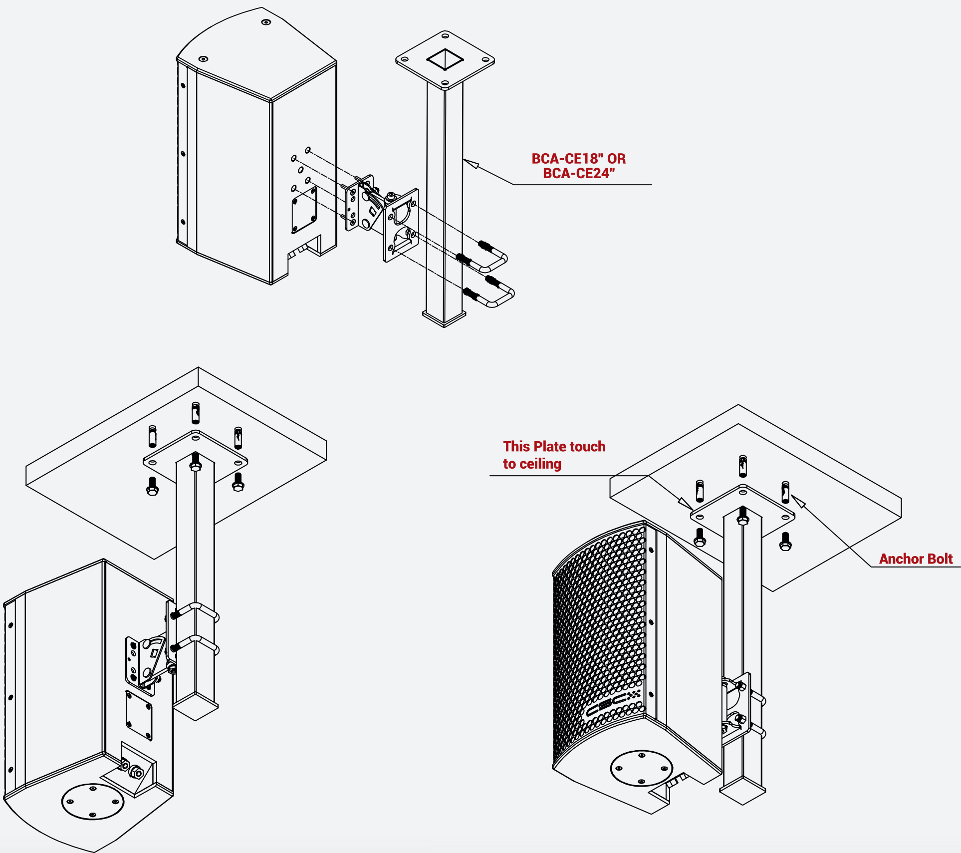
The illustration above displays the ceiling mounting arrangement for the CC8 loudspeaker and identifies the essential hardware supplied.
